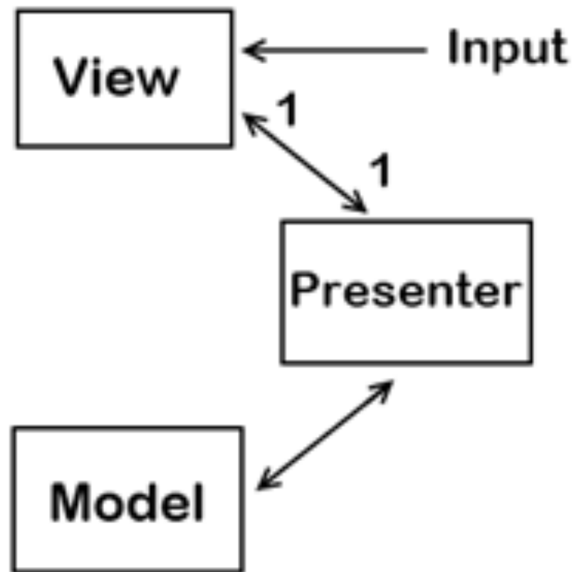
MVP
