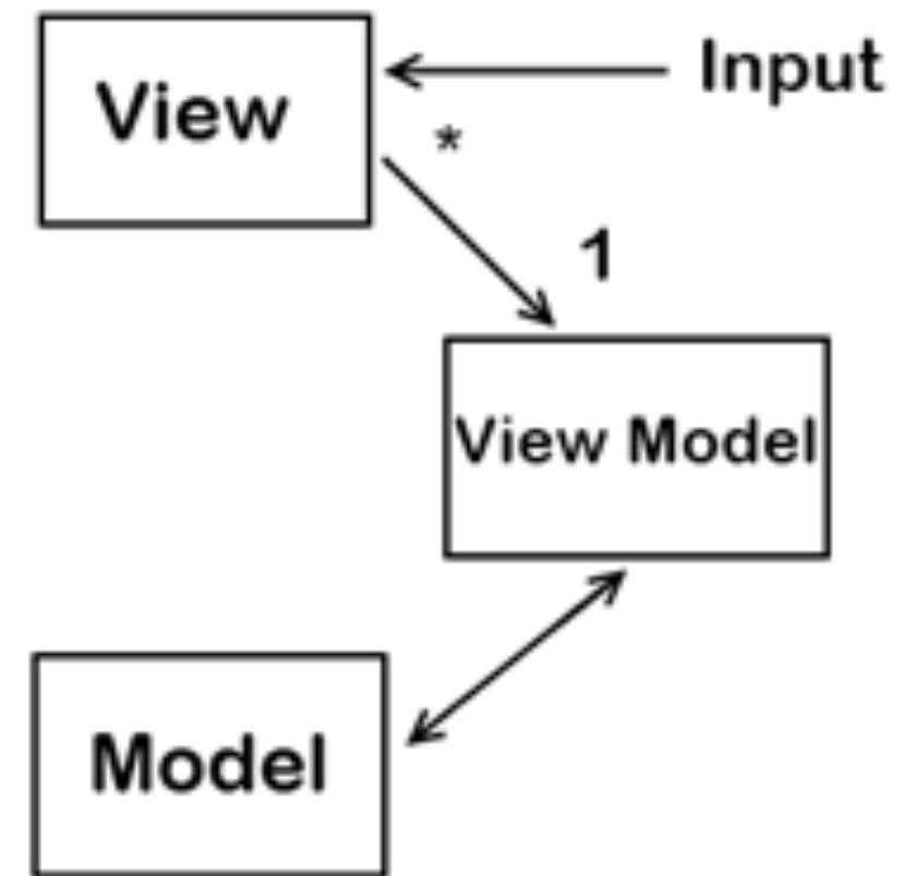
MVVM
